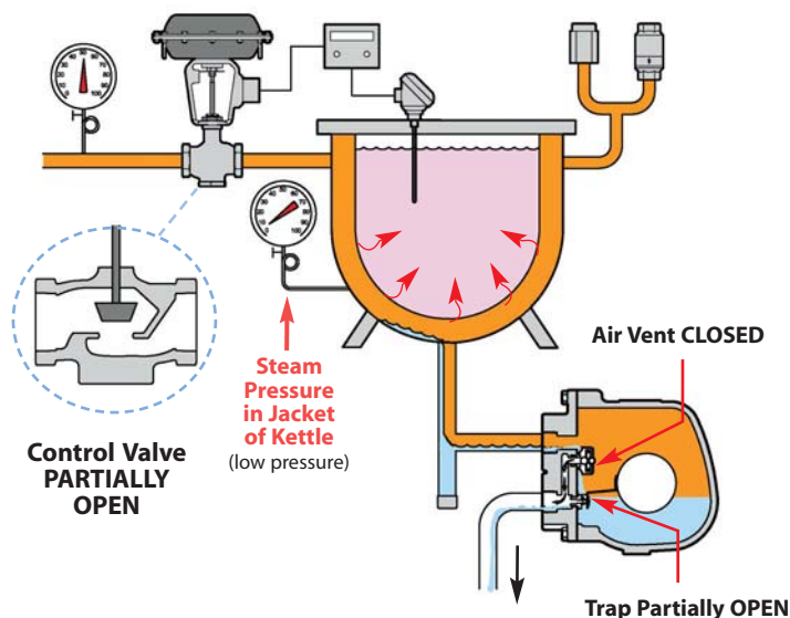
Process Liquid is nearing Set Temperature
