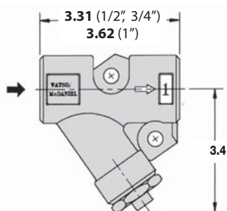
UC450SR (Strainer)
