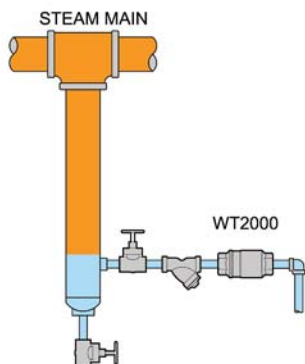
Steam Main Drip
