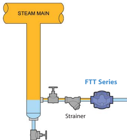
Steam Main Drip Application
