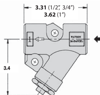
UC450SL (Strainer)
