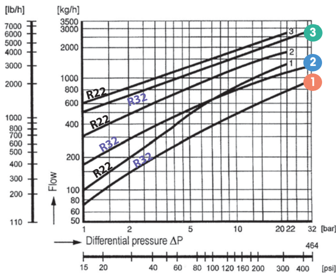
WPN-40 with R22 & R32 Controller
