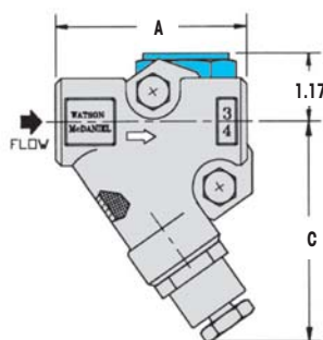
UC450SBR CONNECTOR
